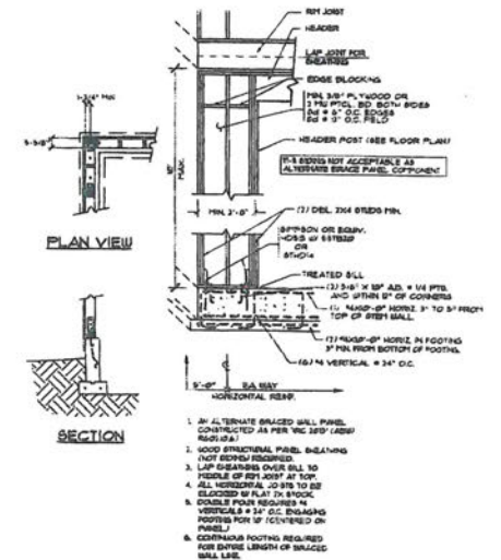
ABW ALTERNATE BRACE WALL DETAIL
