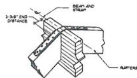
SIMPSON' LSTA DETAIL NOT TO SCALE
